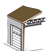
LOW HEADROOM front mount torsion
